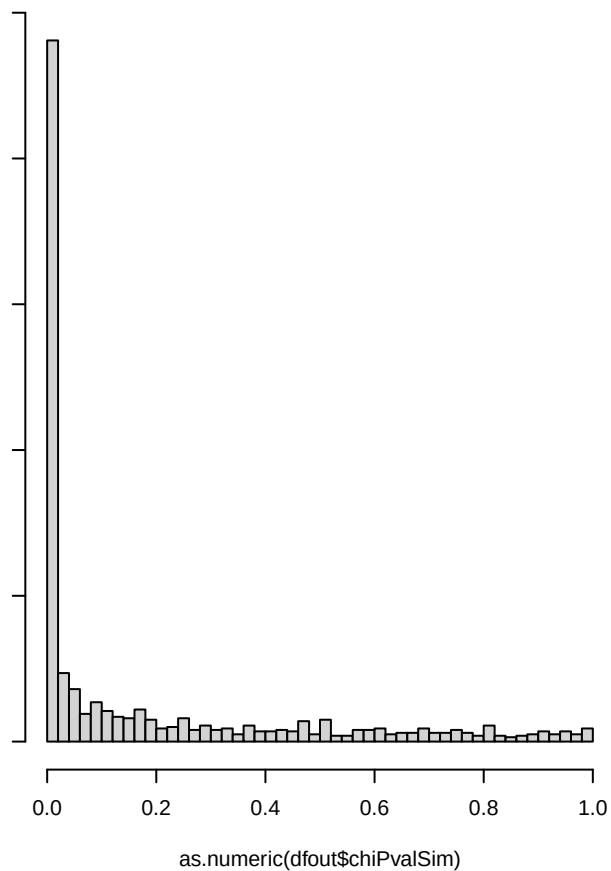
chisq SimPval distribution, numsig: 550 /1000
